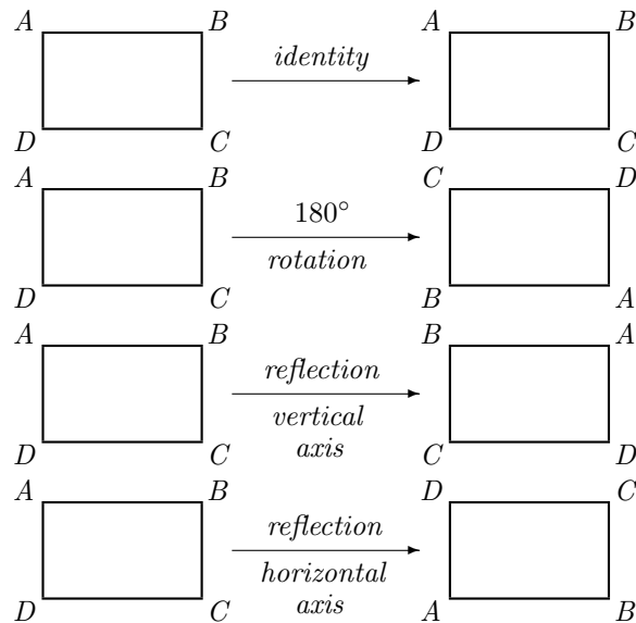
Figure 2.1. Rigid motions of a rectangle
