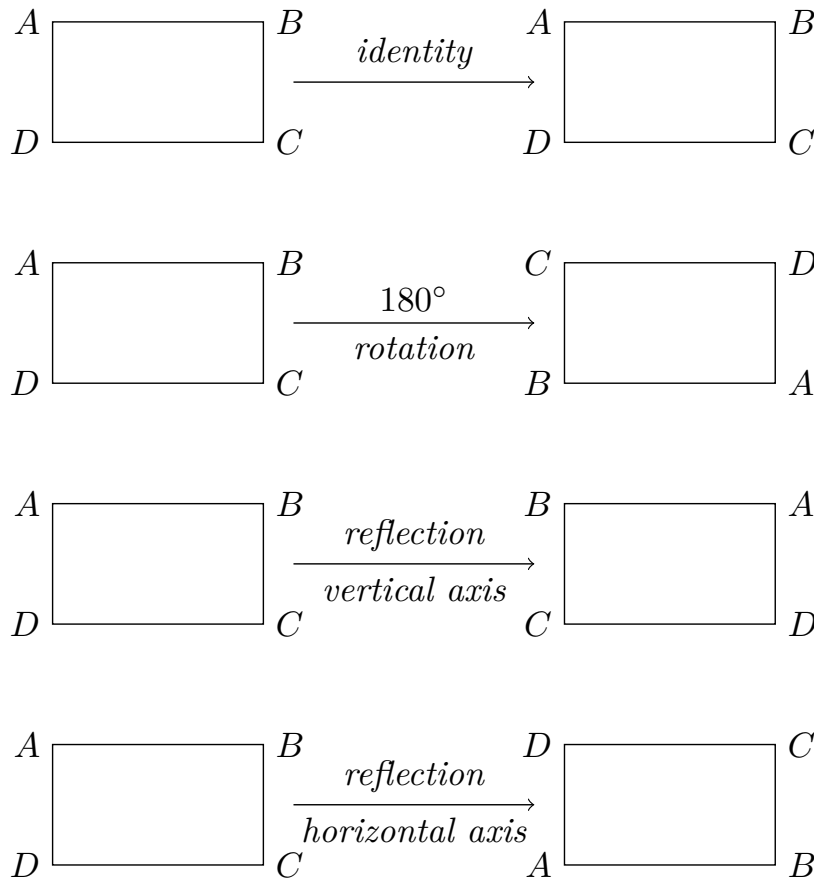
Figure 3.5 Rigid motions of a rectangle
