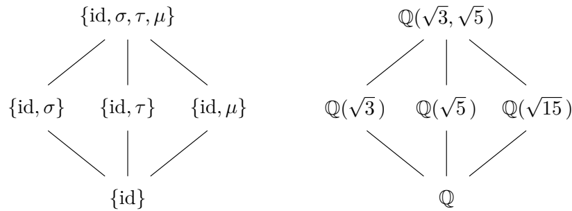
Figure 23.21 G(\mathbb{Q}(\sqrt{3}, \sqrt{5})/\mathbb{Q})
