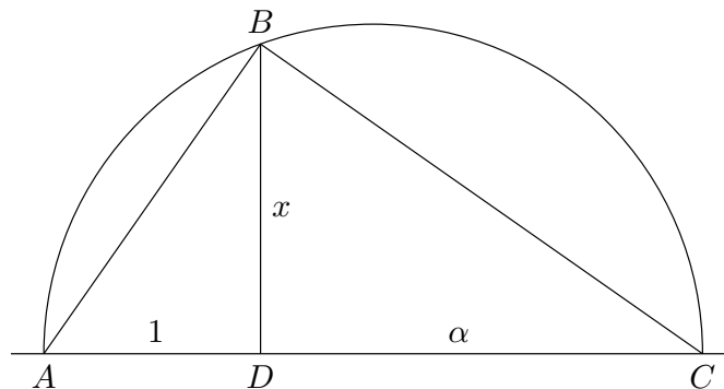
Figure 21.38 Construction of roots
