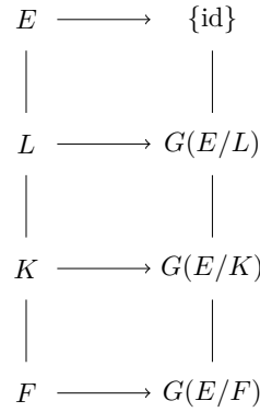
Figure 23.23 Subgroups of G(E/F) and subfields of E
