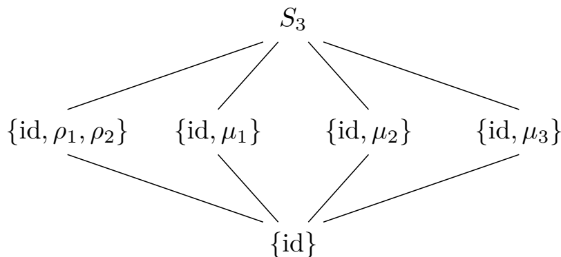
Figure 4.8 Subgroups of S_3
