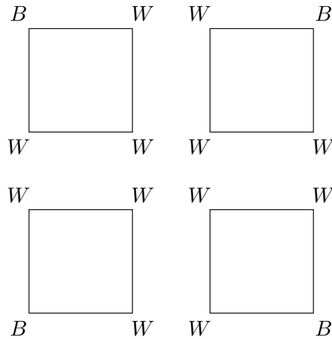
Figure 14.17 Equivalent colorings of square
