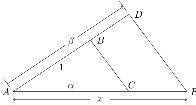
Figure 21.36 Construction of products
