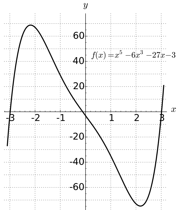
Figure 23.31 The graph of f(x) = x^5 - 6x^3 - 27x - 3
