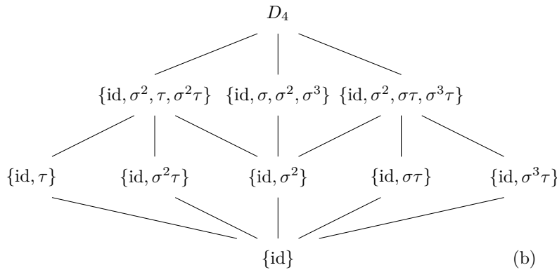
Figure 23.25 Galois group of x^4 - 2
