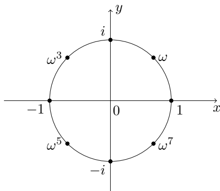
Figure 4.27: 8th roots of unity
