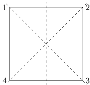
Figure 5.4. The group D_4
