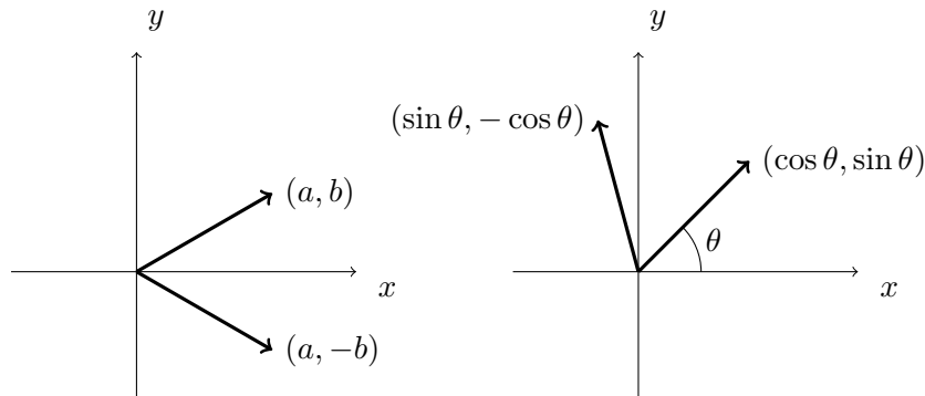
Figure 12.2. O(2) acting on \mathbb{R}^2
