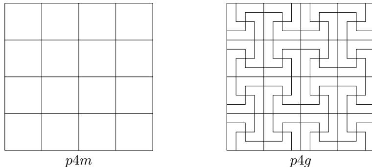
Figure 12.9. The wallpaper groups p4m and p4g
