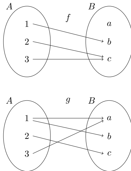
Figure 1.1. Mappings
